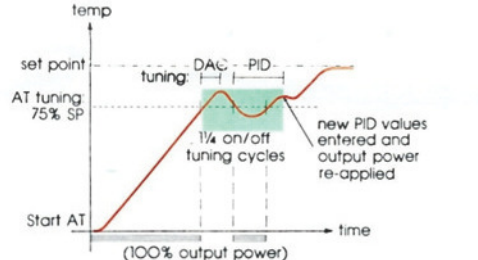
Fig. 1 Autotune AT
